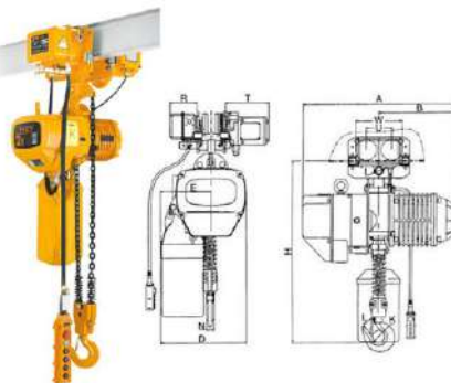
Electric Chain Hoists
